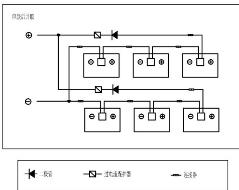
Fig.10 Electrical diagram of series and parallel lines
